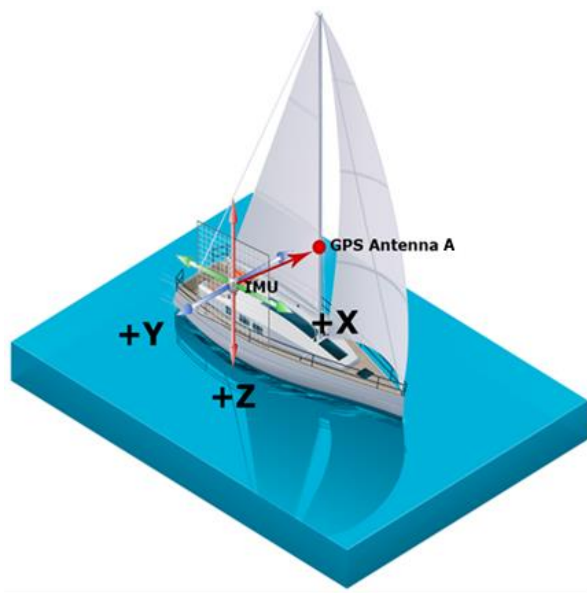
GNSS Antenna A Offset
