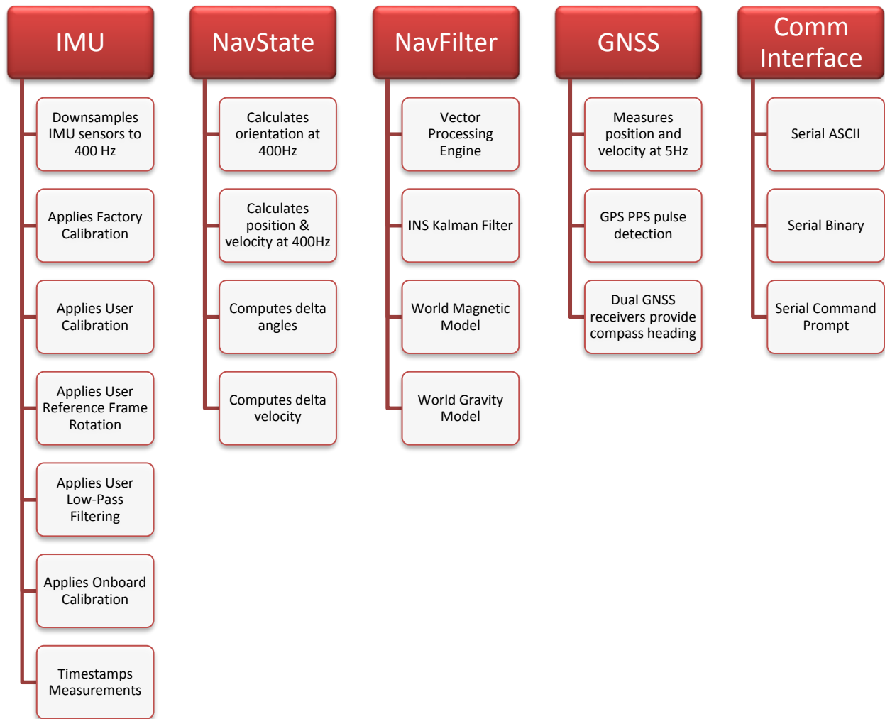
VN-300 Software Architecture
