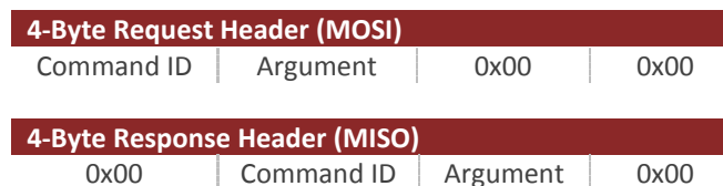
Figure 3 - Packet Headers
